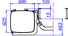
Vista A / View A
