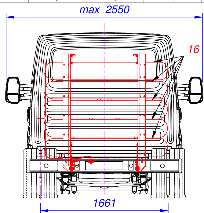
Dettaglio rack verticale senza paratia. Vertical rack detail without bulkhead.
