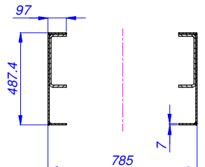
SECTION F-F SCALE 1:20
