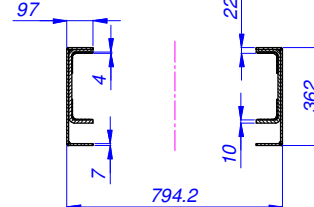
SECTION C-C SCALE 1:20
