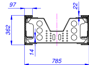
SECTION E-E SCALE 1:20
