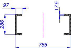
SECTION G-G SCALE 1:20
